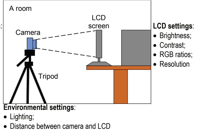
Fig. 3 Our Image Recapturing Environment where the Tunable Settings to Achieve Better Quality of Recaptured Images are Highlighted
